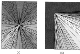
Figure A.3.1. The polyhedron \Pi for SL_2(\mathbb{Z}) . In (a) we see \Pi from the origin, in (b) from the side. The small triangle at the right center of (a) is the facet with vertices \{q(e_1), q(e_2), q(e_1 + e_2)\} , where \{e_1, e_2\} is the standard basis of \mathbb{Z}^2 . In (b) the x -axis runs along the top from left to right, and the z -axis runs down the left side. The facet from (a) is the little triangle at the top left corner of (b).
