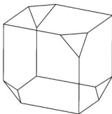
Figure A.3.4. The Soulé cube.
